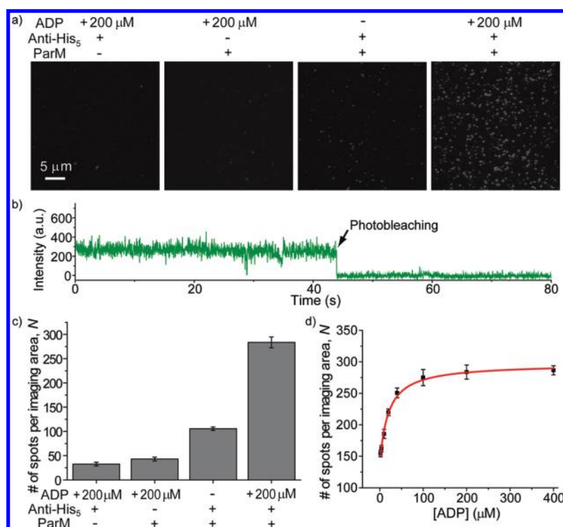
Figure 2. (a) Representative TIRF images taken in the absence and presence of ParM with the indicated ADP concentrations and surface conditions (penta-His-antibody coated surface or not). (b) A representative fluorescence-intensity time trace for the molecules in the absence of ADP, showing steady and continuous fluorescence over time. (c) The average number of fluorescent spots per imaging area determined in the absence and presence of ParM and/or ADP. (d) The average number of fluorescence spots per imaging area as a function of the ADP concentration. The red line is the fit to a hyperbola.
