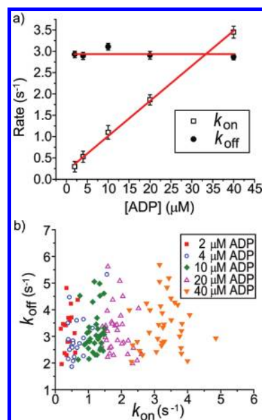
Figure 4. (a) The transition rates between the quenched and unquenched states at five ADP concentrations. The best fit horizontal was performed for k_{\text{off}} and the best linear fit was performed for k_{\text{on}} . (b) Scatter plots of the transition rates among many different individual molecules at five ADP concentrations.
