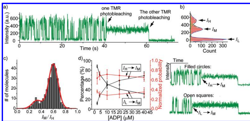
Figure 5. (a,b) A representative fluorescence-intensity time trace for the molecules showing conversion from two-state dynamics to steady fluorescence and the corresponding fluorescence intensity distribution. (This trace was taken at 20 \mu\text{M} ADP.) (c) Distribution of the ratio I_M/I_H built from 343 molecules that show the type of time trace in (a). The red line is the fit to the sum of two Gaussian peaks. (d) The percentages of the molecules that convert from the unquenched to the I_M state or from the quenched to the I_M state when the molecule switches from a dynamic to a steady phase at five ADP concentrations with calculated probabilities normalized to the average dwell time of the state before the conversion. The example conversion traces (from I_H to I_M , from I_L to I_M ) are shown in the right.
