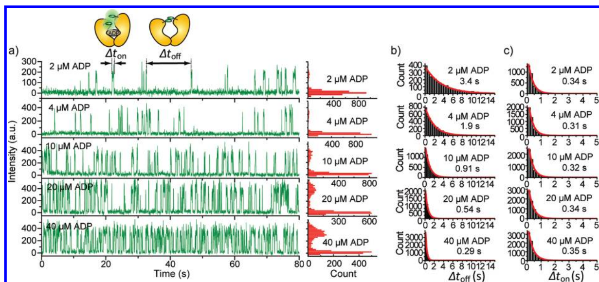
Figure 3. (a) Representative fluorescence-intensity time traces for the molecules showing two-state dynamics at five different ADP concentrations with the corresponding fluorescence intensity distributions. (b,c) Dwell time analysis for the two states respectively at the five ADP concentrations. The dwell time histograms were built from 50 to 100 molecules at each ADP concentration. The red lines are the single exponential fits to the dwell time histograms. \tau_{\text{on}} or \tau_{\text{off}} obtained from the fit is shown next to each histogram.
