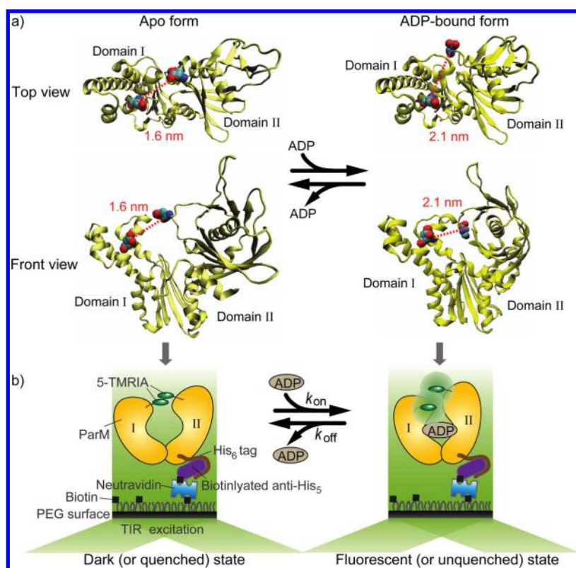
Figure 1. (a) The top and front views of ParM apo structure (left, PDB entry 1MWM) and the ADP-bound ParM structure (right, PDB entry 1MWK). The positions of the two cysteine mutations and the distance between them are shown (1.6 nm for the quenched state and 2.1 nm for the unquenched state; the distances were measured between cysteine \alpha -carbons). (b) The experimental scheme that shows how the protein is anchored onto the PEG-coated surface through anti-His 6 /His 6 -tag and biotin/neutravidin interactions (also see Experimental Section).
