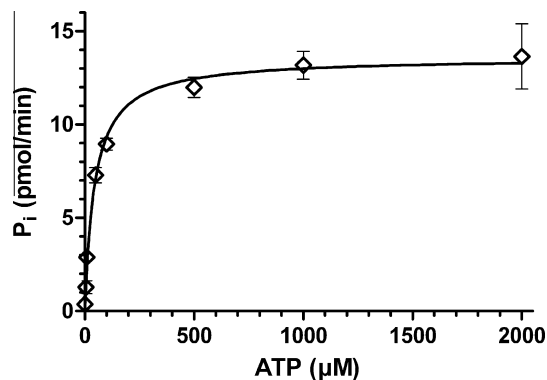
Fig. 3. Michaelis–Menten plot of the intrinsic ATPase activity of ecSecA(W775A) at 22 °C. Initial rates of ATP hydrolysis by ecSecA(W775A) (10 pmol in 50 mM Tris–HCl, 50 mM KCl, 5 mM \text{MgCl}_2 , 0.4 mg/ml BSA, pH 8.0) were measured at different ATP concentrations (0–2 mM) using the malachite green method as described under Experimental procedures. Values are the means of three independent experiments, with error bars representing the standard deviation.
