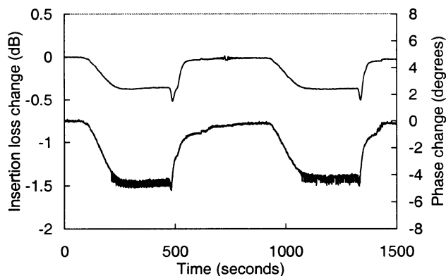
Fig. 5 Change in insertion loss (upper line) and phase (lower line) as a function of time for two cycles of POPC deposition and removal using the pulse mode system.
