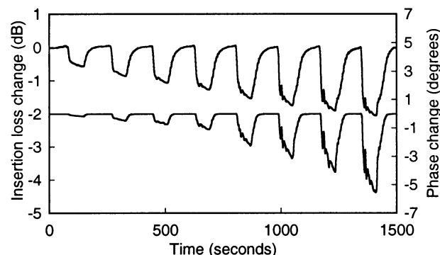
Fig. 3 Change in insertion loss (upper line) and phase (lower line) for a sequence different concentrations of 3350 molecular weight poly(ethylene glycol) solutions using the pulse mode system.
