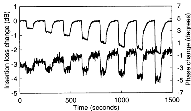
Fig. 2 Change in insertion loss (upper line) and phase (lower line) for a sequence different concentrations of 3350 molecular weight poly(ethylene glycol) solutions using the continuous wave system.
