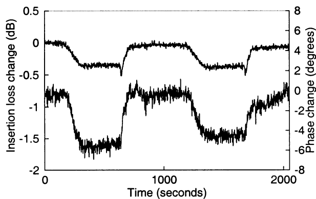
Fig. 4 Change in insertion loss (upper line) and phase (lower line) as a function of time for two cycles of POPC deposition and removal using the continuous wave system.
