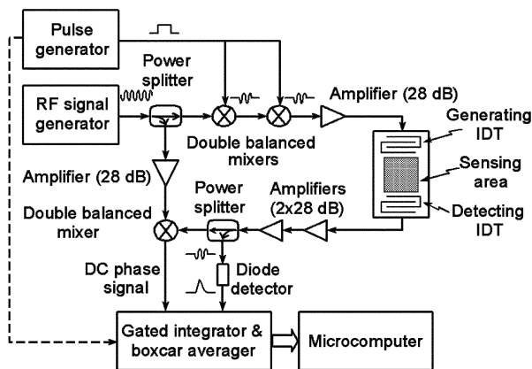
Fig. 1 Schematic diagram of the pulse mode system.
